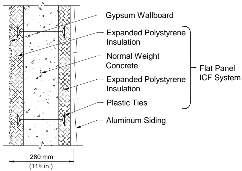
Figure A-8. ICF wall cross-section.
