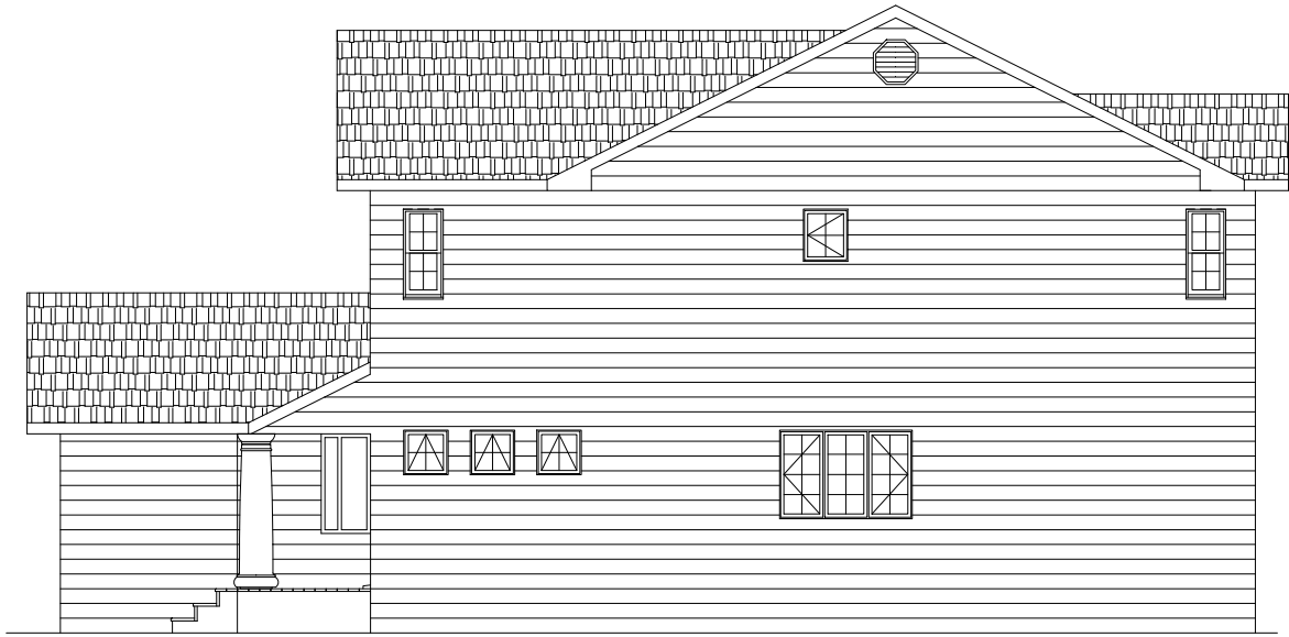
Figure A-5. Right elevation.
